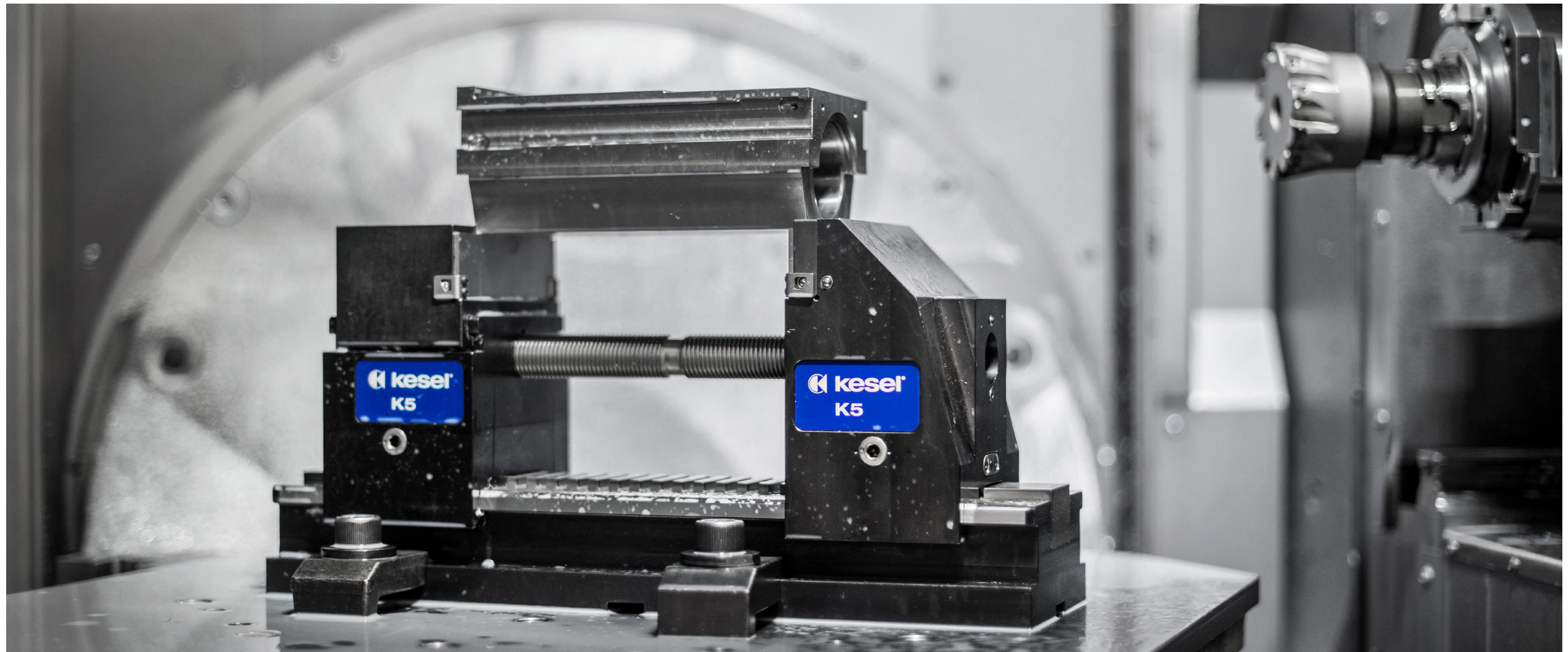
Der Kesel 5-Achs-Spanner K5 The Kesel K5 5-Axis vise
